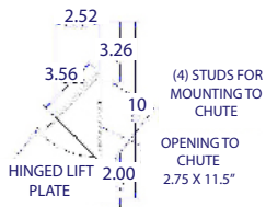
STEEL CHUTE PROFILE
