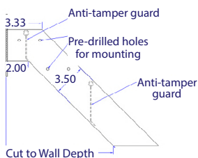
STEEL CHUTE PROFILE
