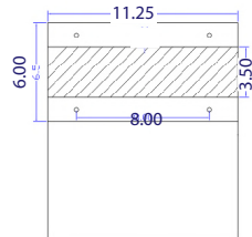
STEEL CHUTE PLAN
